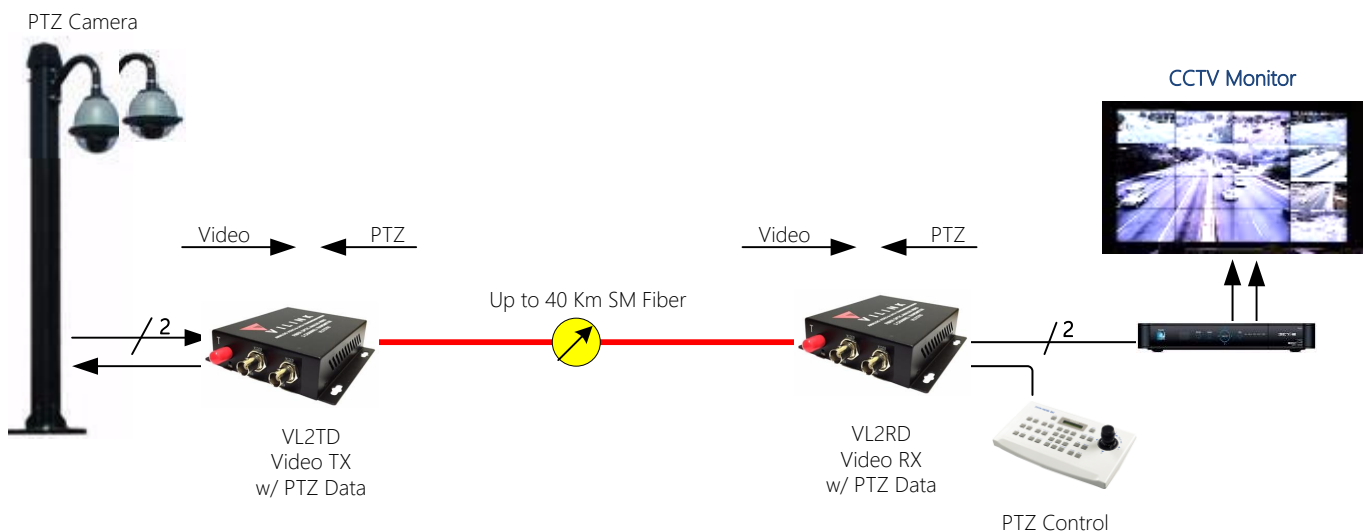
Typical VL2 Application
