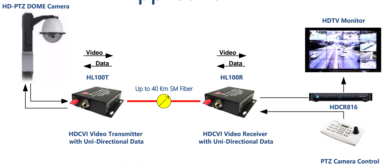
Typical HL100T & HL100R In Traffic Monitoring Application
